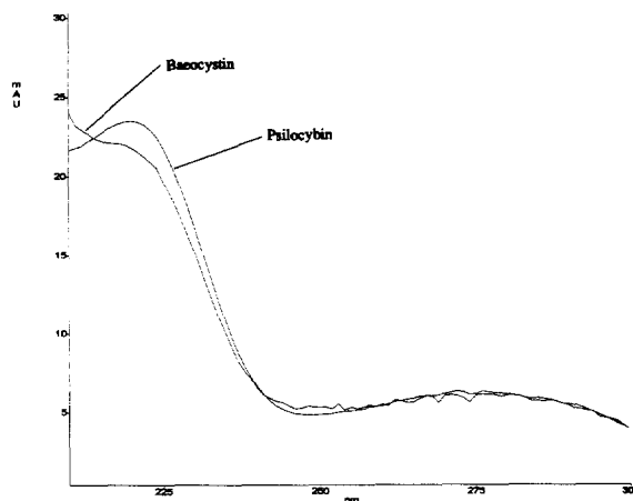
Fig. 5. UV spectra of psilocybin and baeocystin obtained during capillary zone electrophoresis. Buffer: 10 mM borate-phosphate adjusted to pH 11.5.
